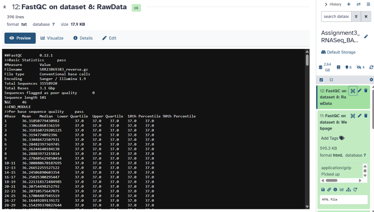
Figure 5. Raw Data Output of the FastQC Analysis for the Reverse Read (Treatment_24hrs_Rep1_R2) Generated Using the FastQC Tool in Galaxy.
